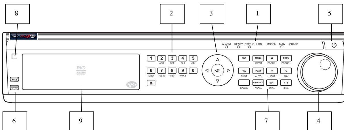
Figure 1.1.5 Front Panel of MAX416
