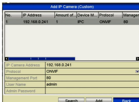
Figure 2.3.1.3 Custom Adding IP Camera Interface
