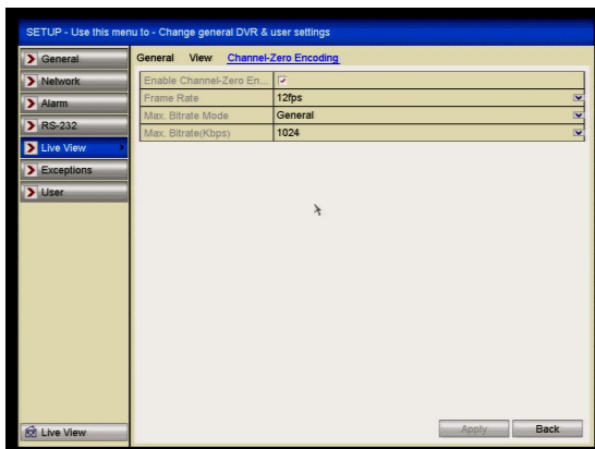
Figure 3.3.1 Live View- Channel-Zero Encoding
