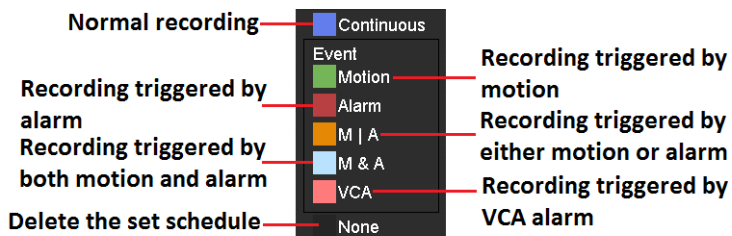
Figure 5.2.6 Descriptions of the Color Icons
