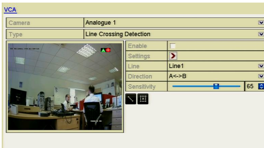
Figure 8.5.1 VCA Alarm Setting Interface
