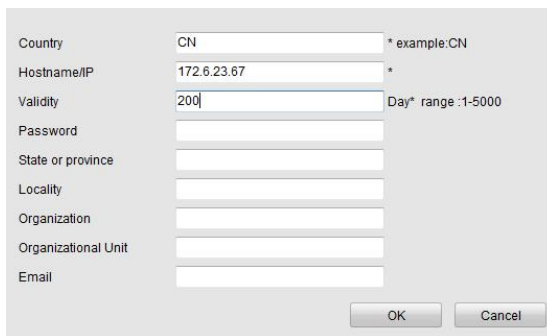
Figure 9.2.7.2 Create Self-signed Certificate
