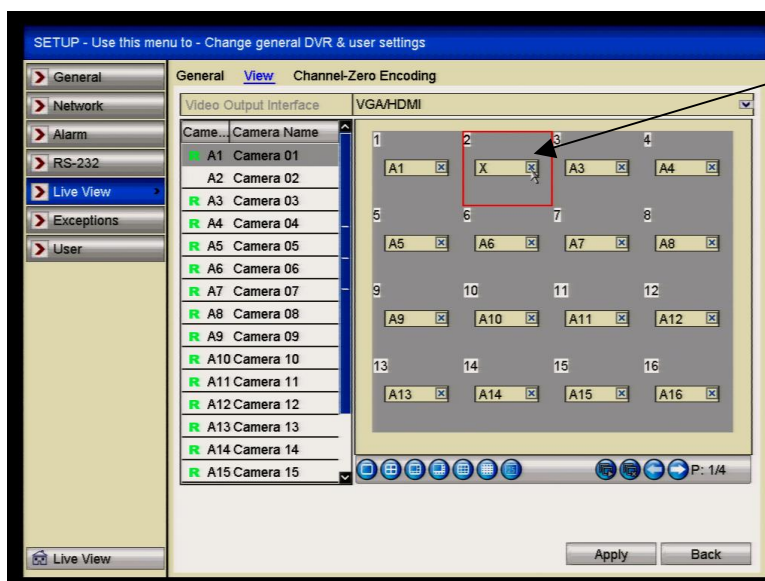
Figure 3.4.2 Live View- Camera Order
