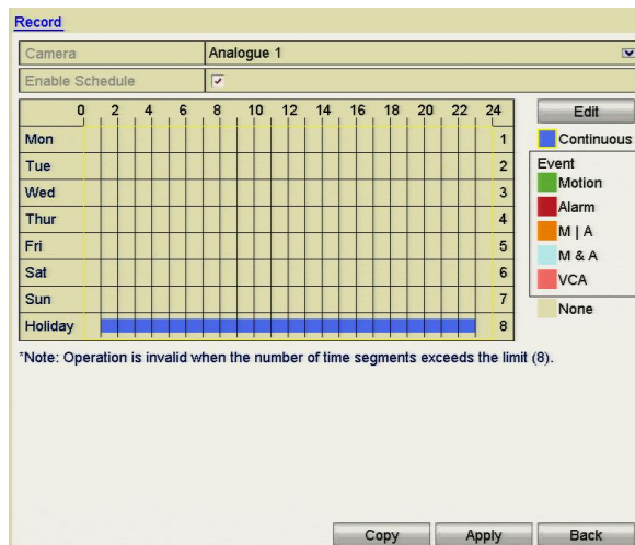
Figure 5.7.3 Edit Schedule- Holiday
