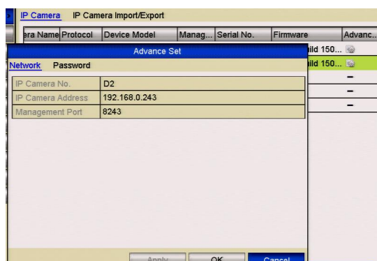
Figure 2.3.2.2 Network Configuration of the Camera
