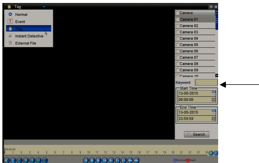
Figure 6.1.4.3 Video Search by Tag
