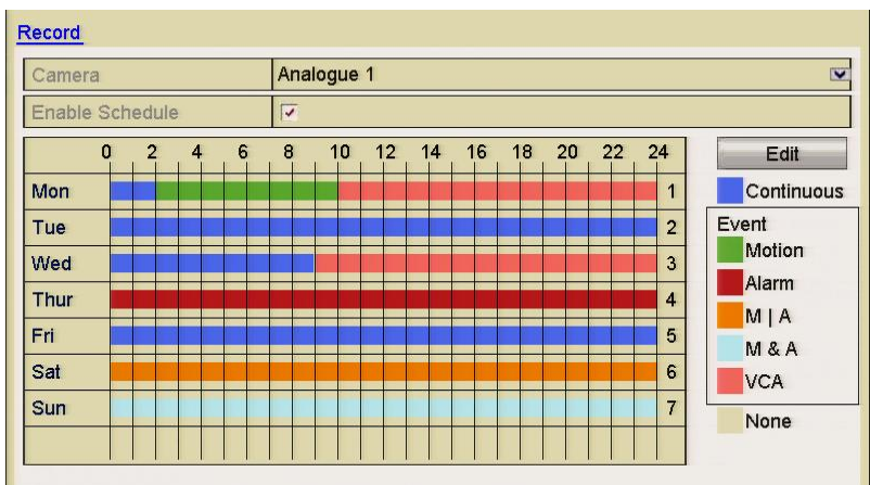
Figure 5.2.5 Draw the Schedule
