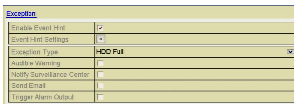
Figure 8.7.1 Exception Settings Interface
