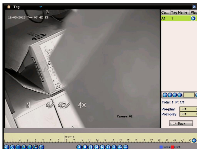
Figure 6.1.4.4 Playback by Tag Interface
