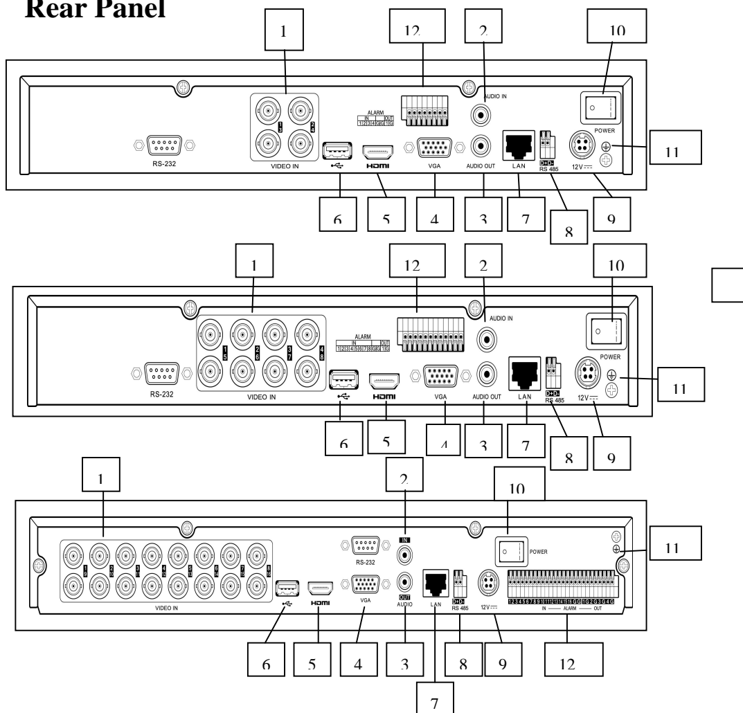
Figure 1.5.1 MEGA204 / MEGA208 / MEGA216
