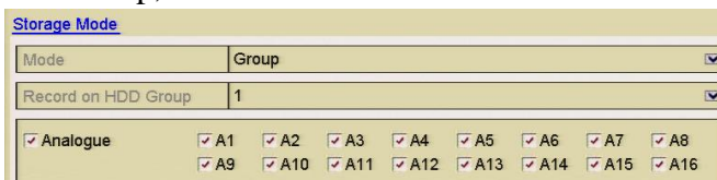
Figure 10.4.1.1 Storage Mode Interface
